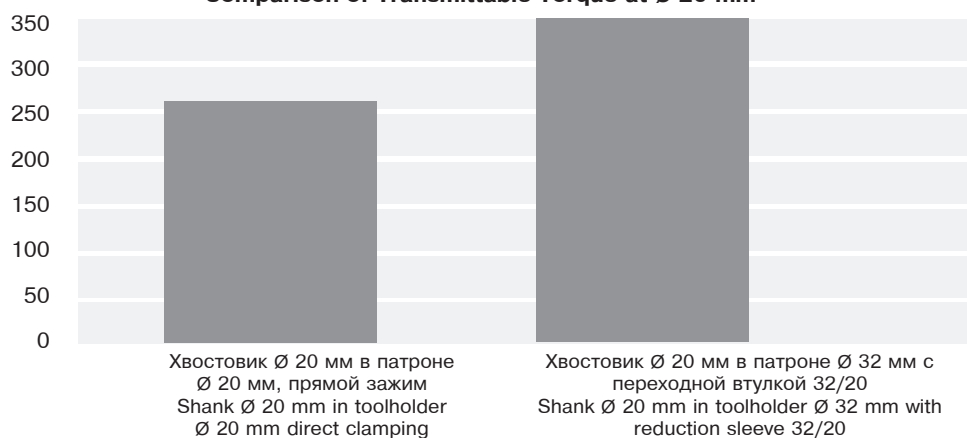
Comparison of Transmittable Torque at \varnothing 20\text{ mm}
